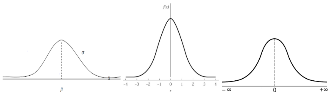
Figure 3.2 Normal Distribution
